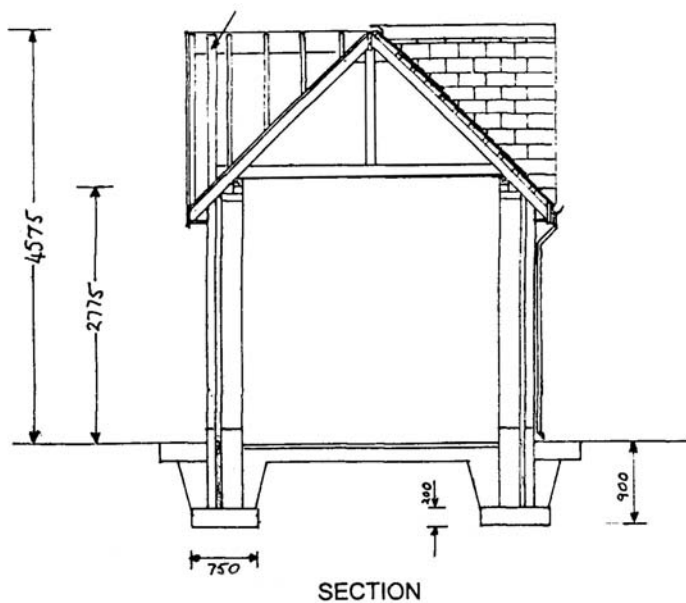
Figure 9.5.1. Replacement roost for pipistrelles.
